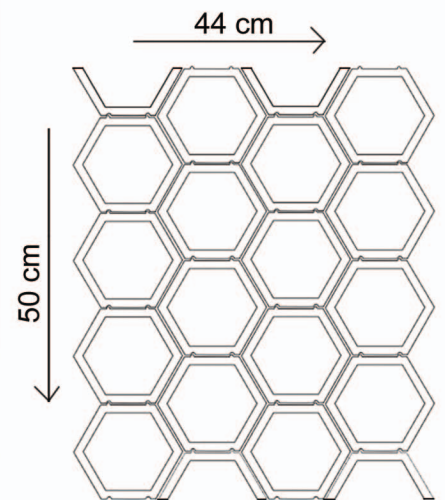
SCHEMA MONTAGGIO - MOUNTING DRAWING
